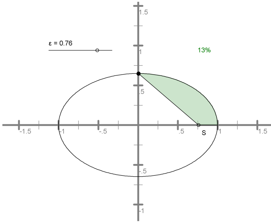
Figure 1: Kepler's Theorem
